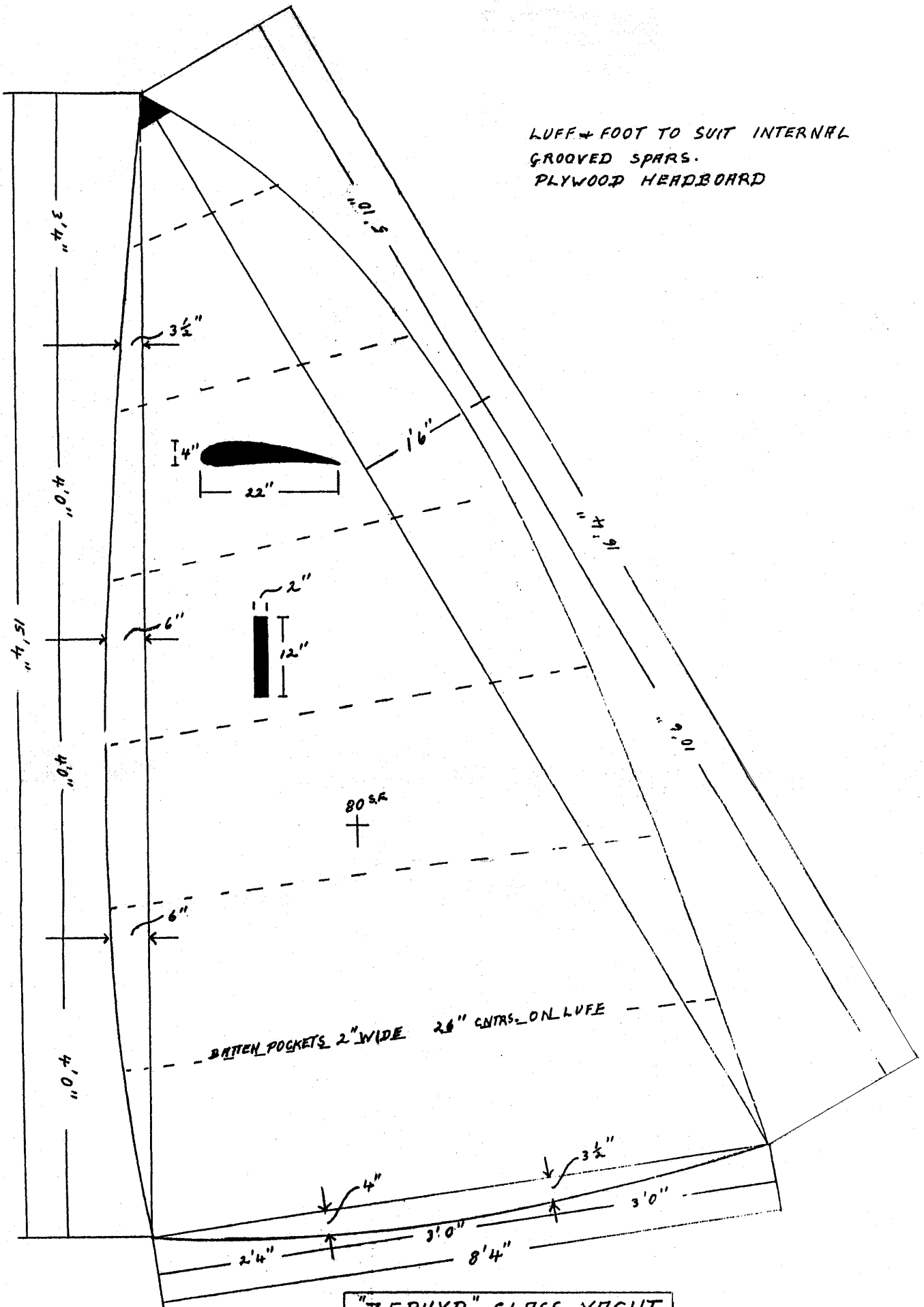
"ZEPHYR" CLASS YACHT
